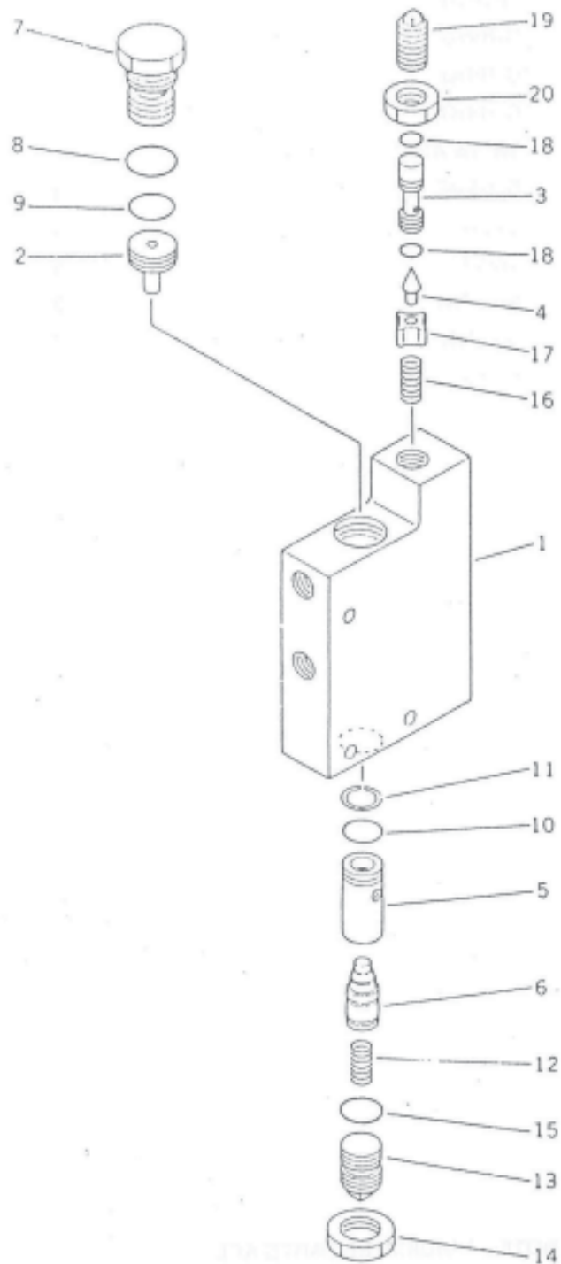
FIG NO.111 PILOT CHECK VALVE (FOR RIPPER) (OPTIONAL)
