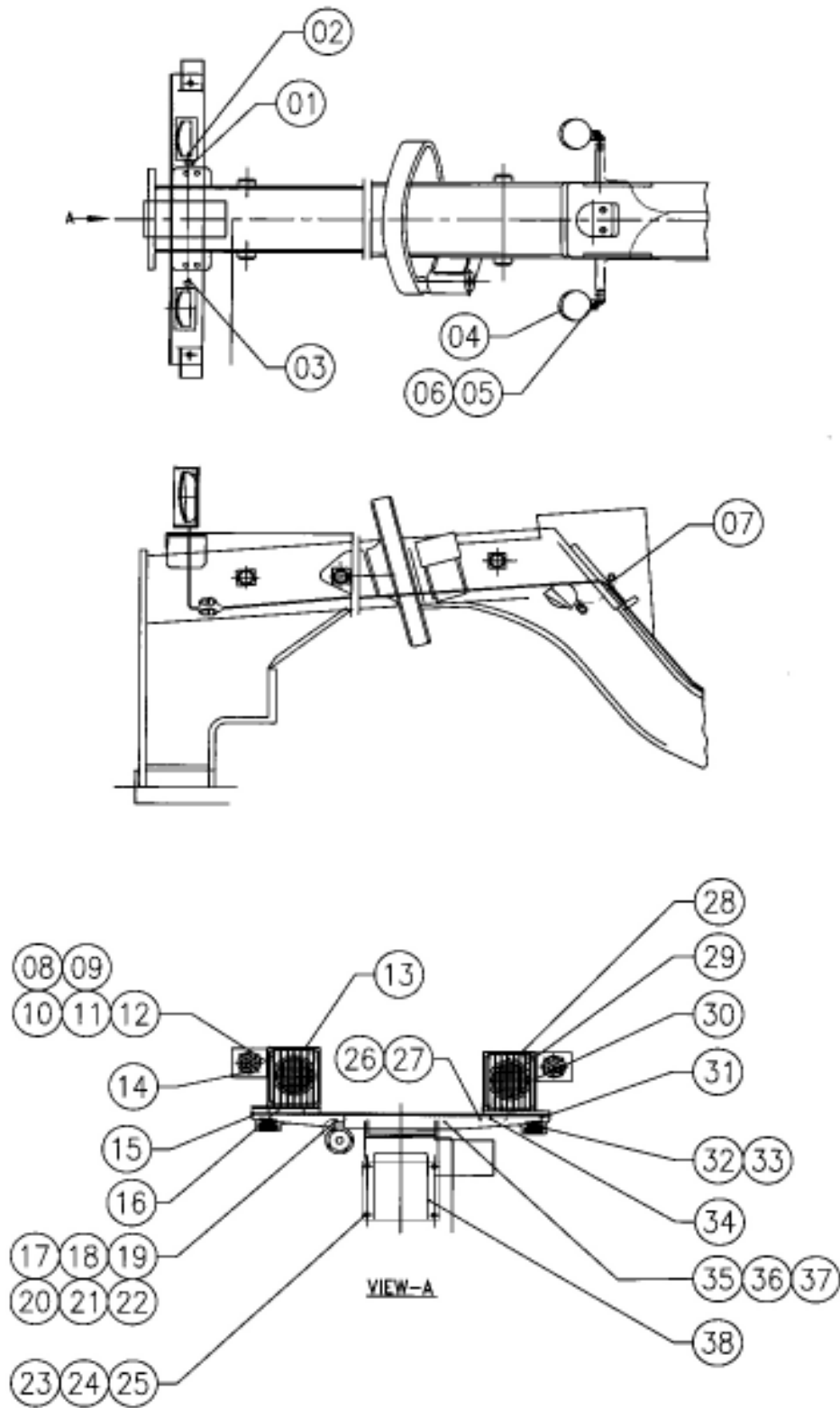
FIG NO. 14 ELECTRICAL SYSTEM (FRONT)
