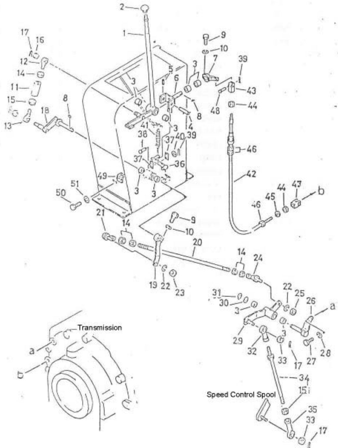
FIG NO. 42 HYDROSHIFT TRANSMISSION CONTROL (2/2)
