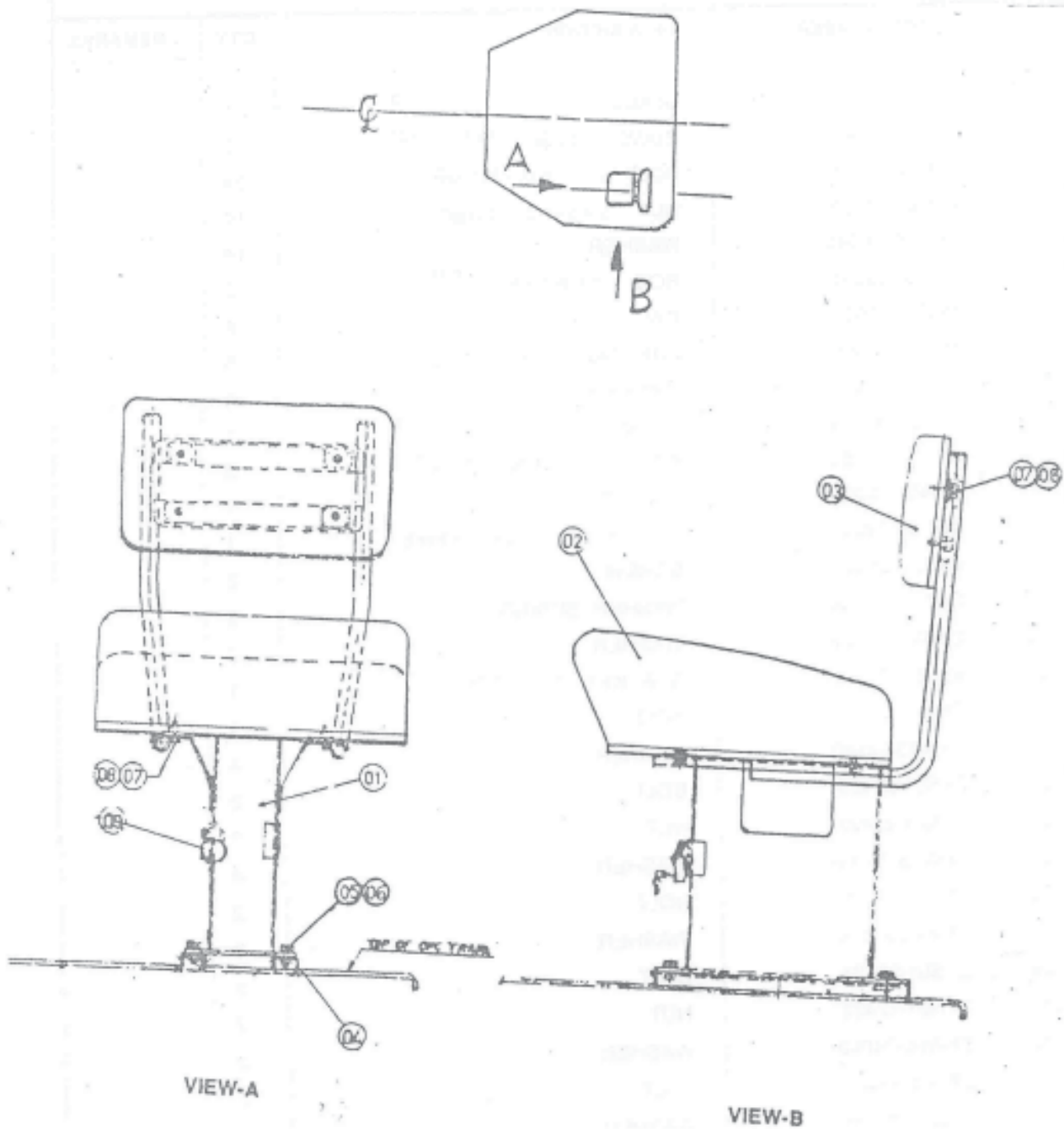
FIG NO.148 INSTALLATION & ASSY OF AUXILLARY SEAT
