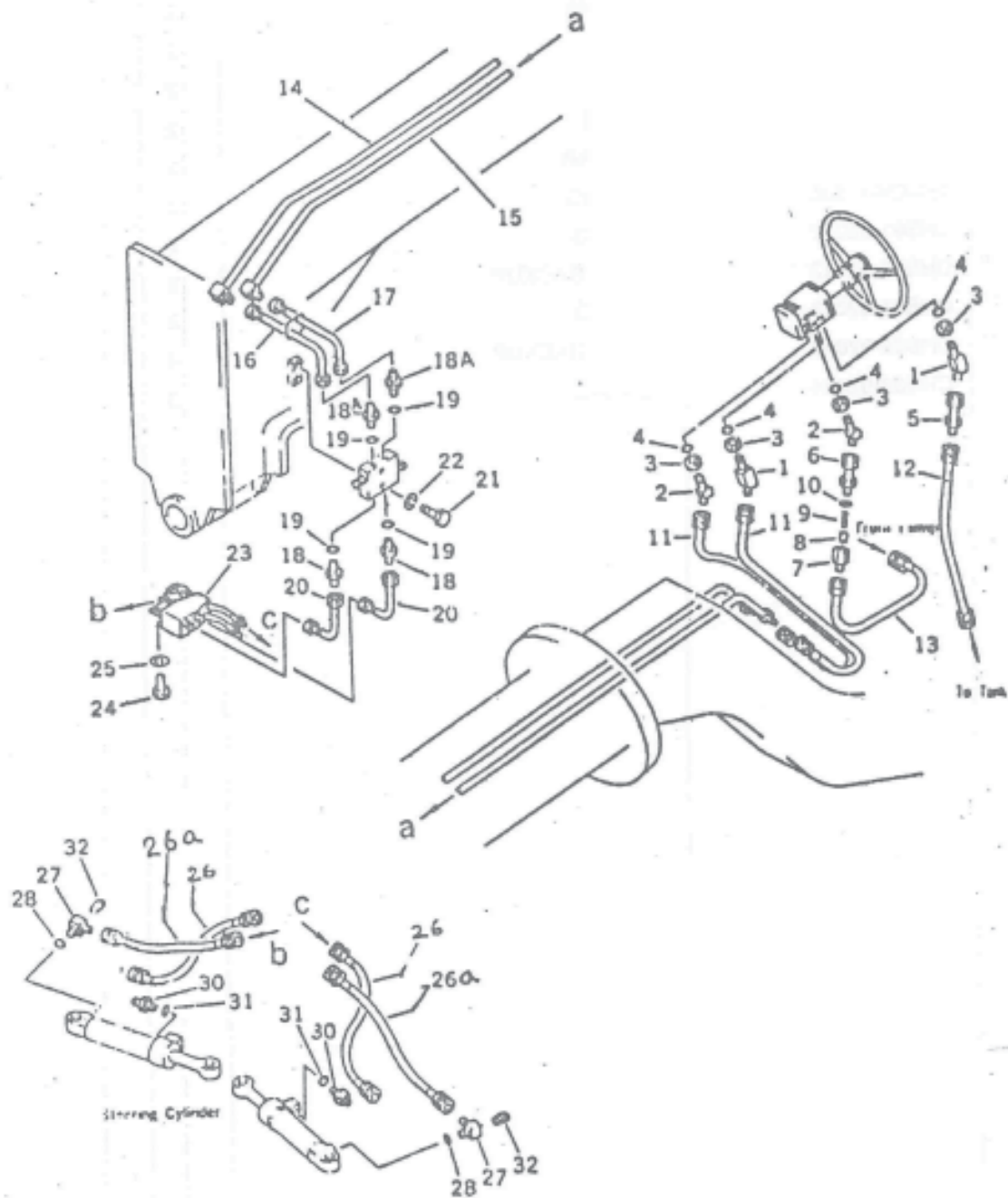
FIG NO.70 STEERING PIPING (1/2)
