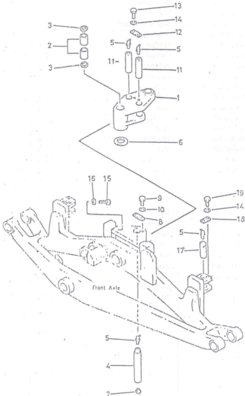
FIG NO. 65 PITMAN ARM
