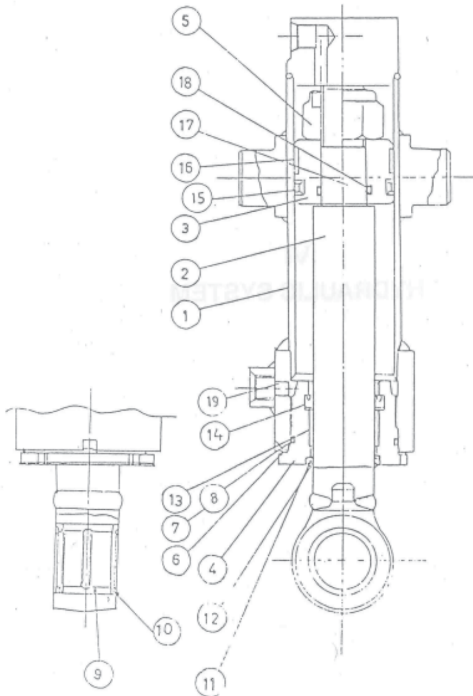
FIG NO. 83 BLADE SHIFT CYLINDER
