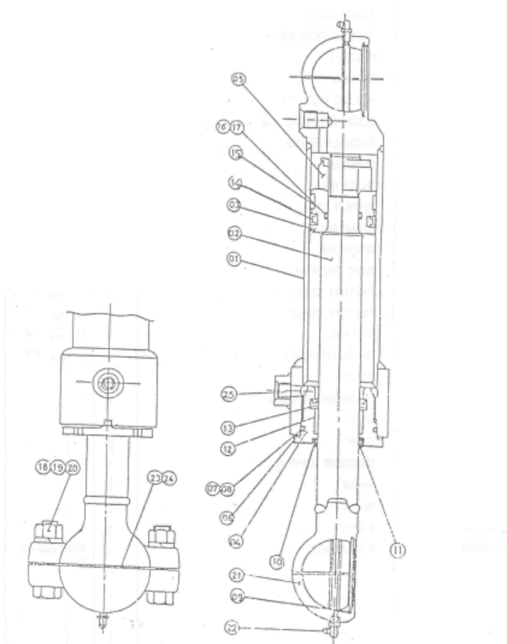
FIG NO. 95 DRAW BAR SHIFT CYLINDER
