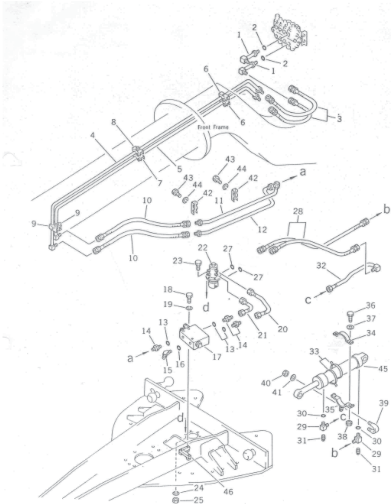
FIG NO.121 POWER TILT BLADE PIPING(OPTIONAL)
