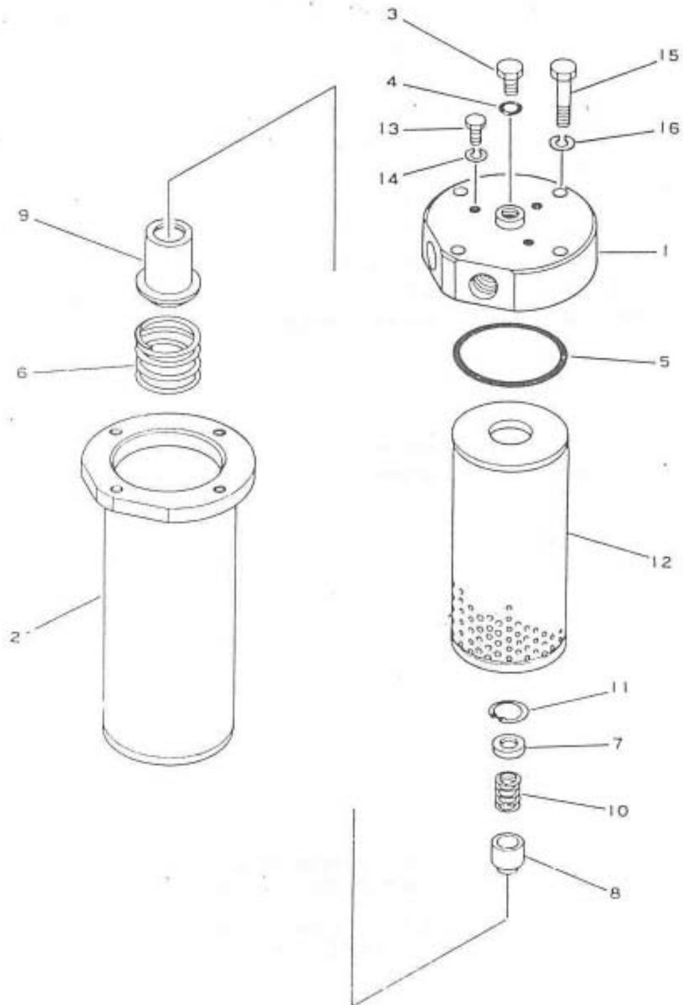
FIG NO.38 HYDROSHIFT TRANSMISSION FILTER
