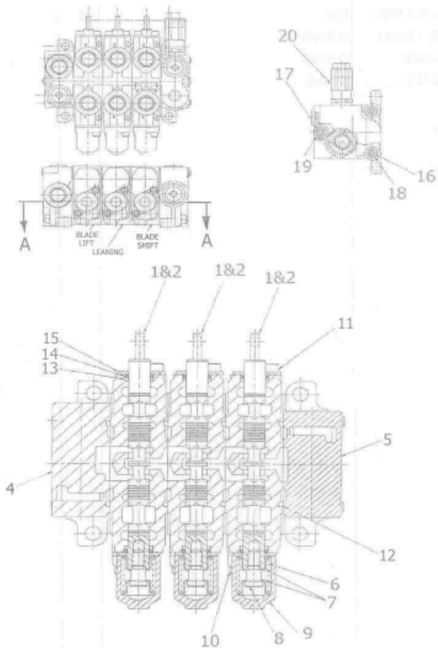
SECTIONAL VIEW
