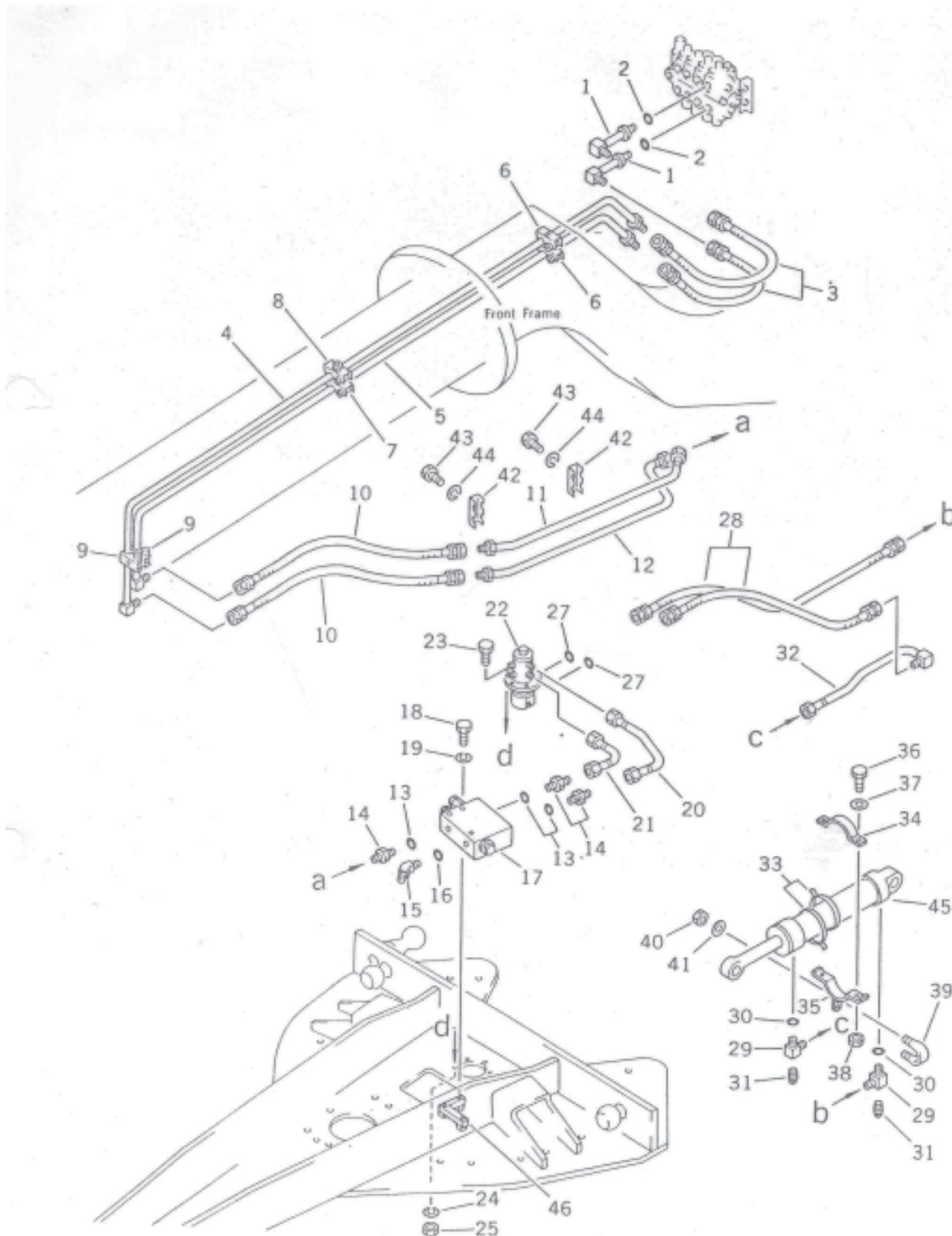
FIG NO.121 POWER TILT BLADE PIPING(OPTIONAL)
