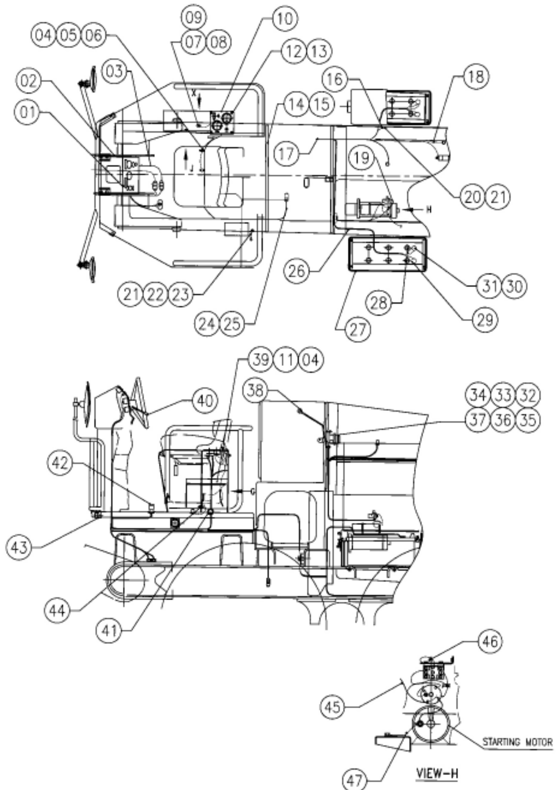
FIG NO. 15 ELECTRICAL SYSTEM (MIDDLE)
