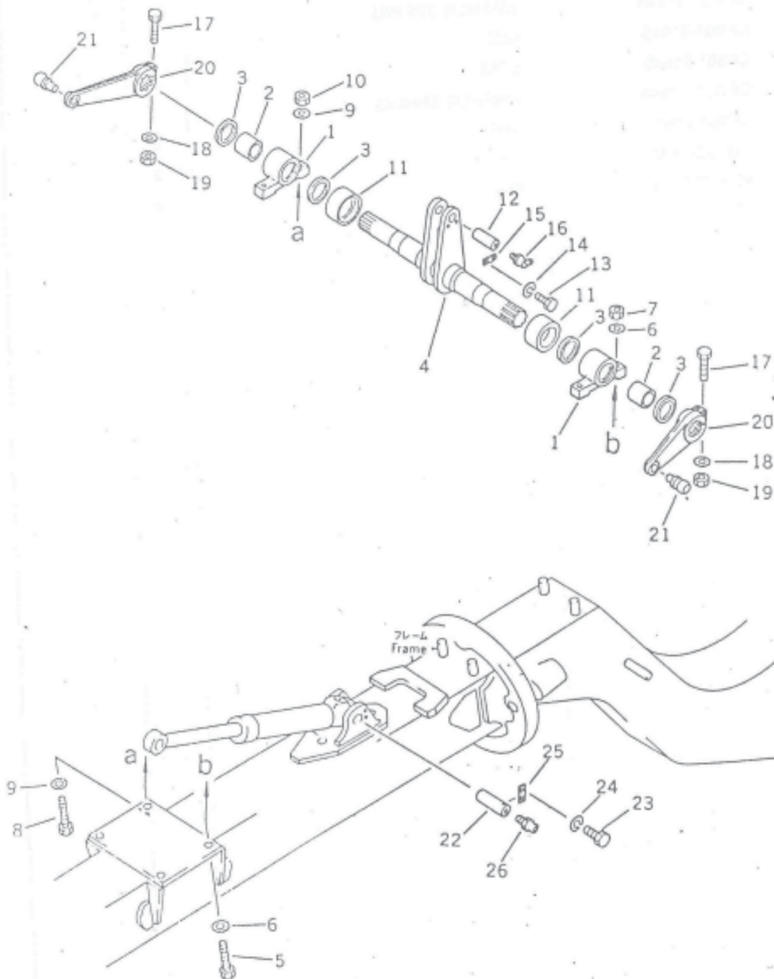
FIG NO.143 SCARIFIER LIFTER (OPTIONAL)
