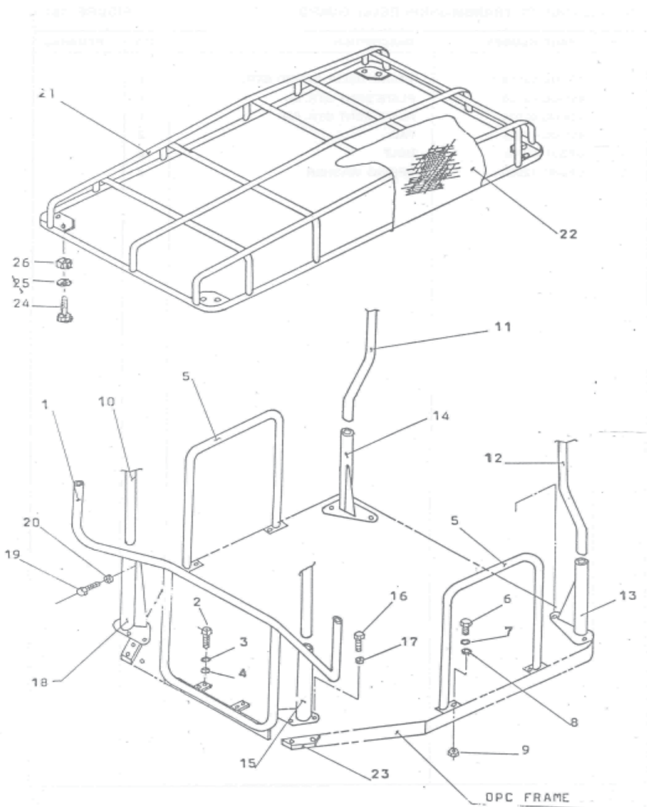
FIG NO.152 CANOPY
