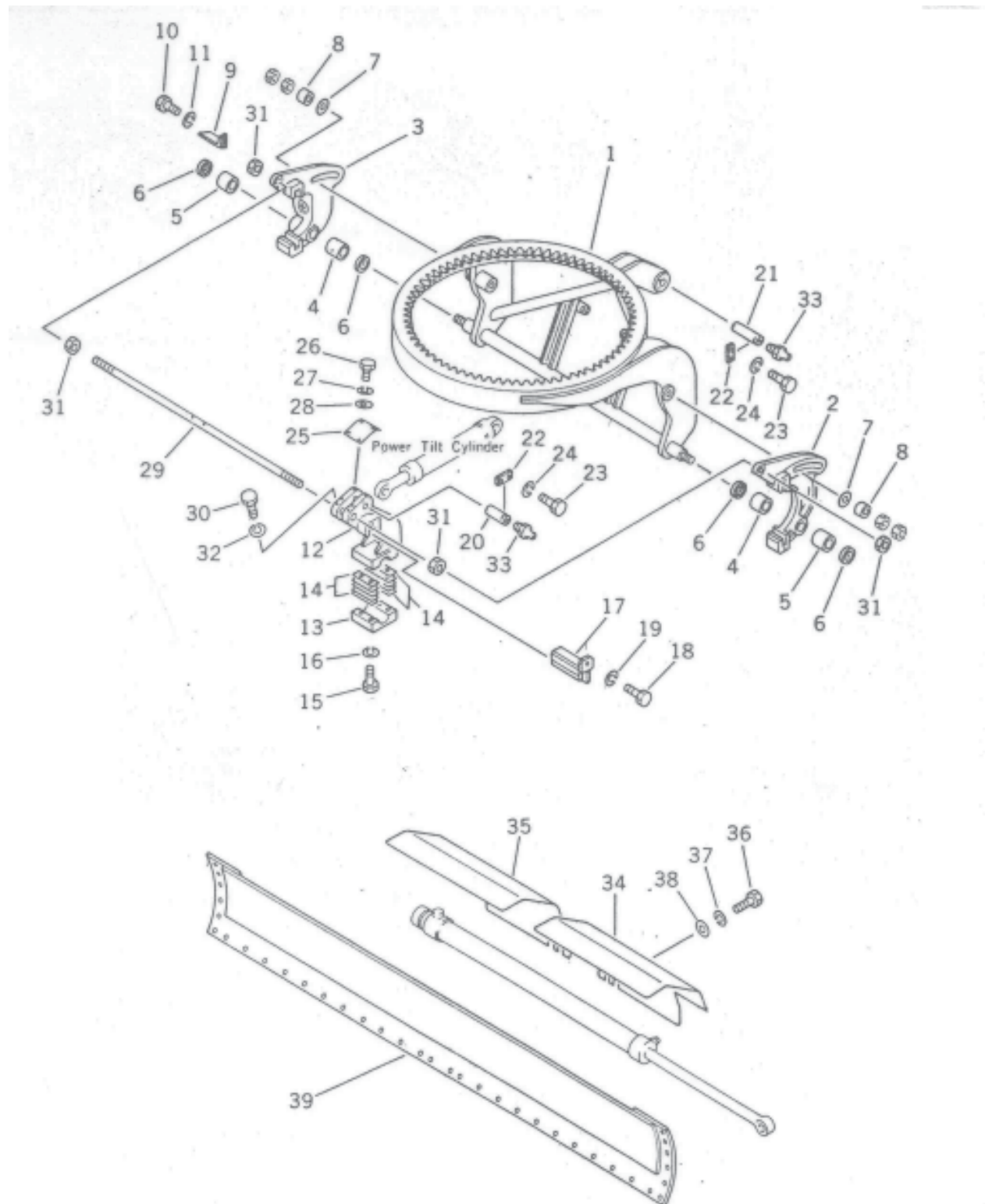
FIG NO.144 SUPPORT FOR POWER TILT BLADE (OPTIONAL)
