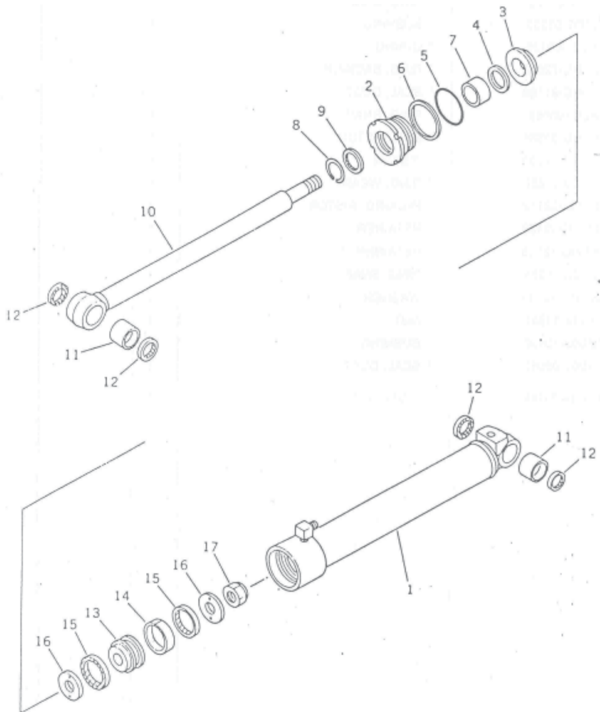
FIG NO. 99 FRONT BLADE CYLINDER (OPTIONAL)
