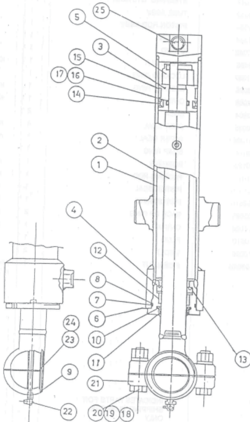
FIG NO. 92 BLADE LIFT CYLINDER
