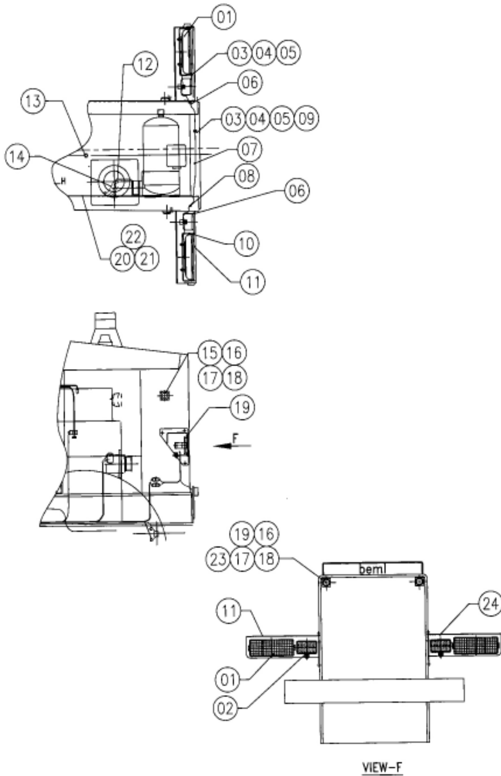
FIG NO.16 ELECTRICAL SYSTEM (REAR)
