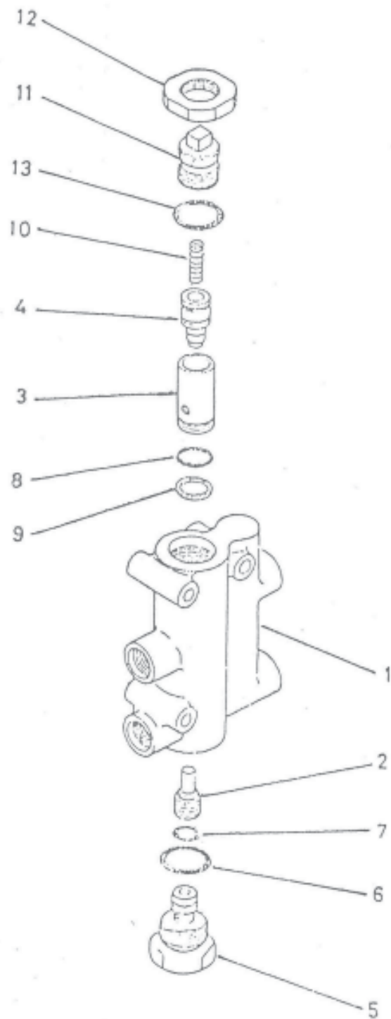
FIG NO.107 PILOT CHECK VALVE (BLADE LIFT RH)
