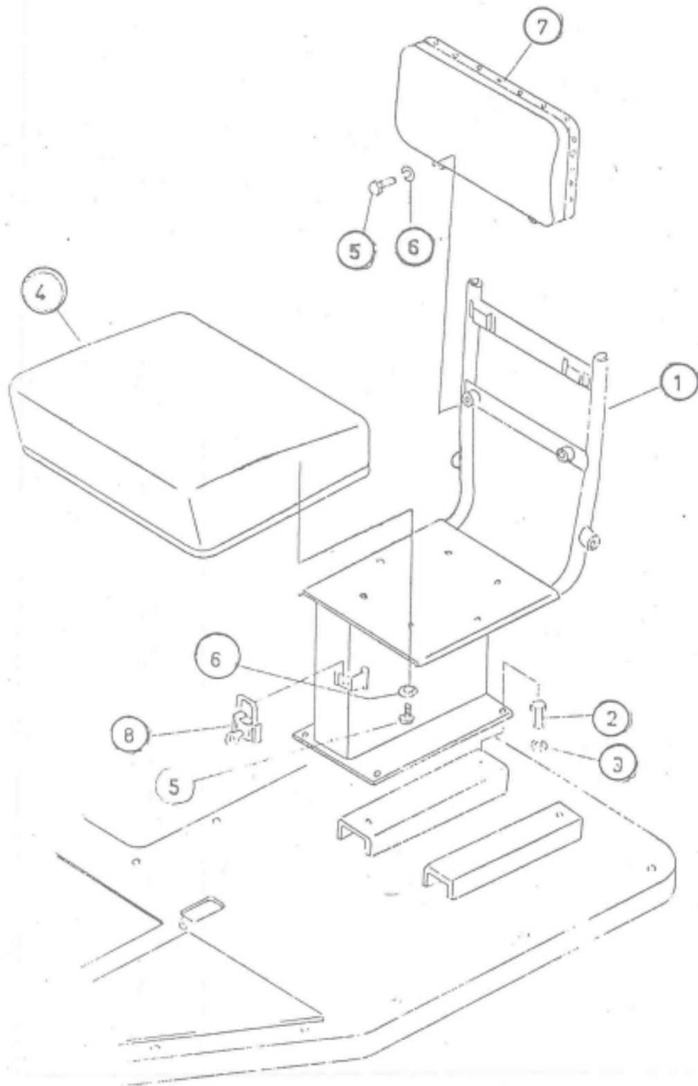
FIG NO.79 AUXILLARY SEAT (OPTIONAL)
