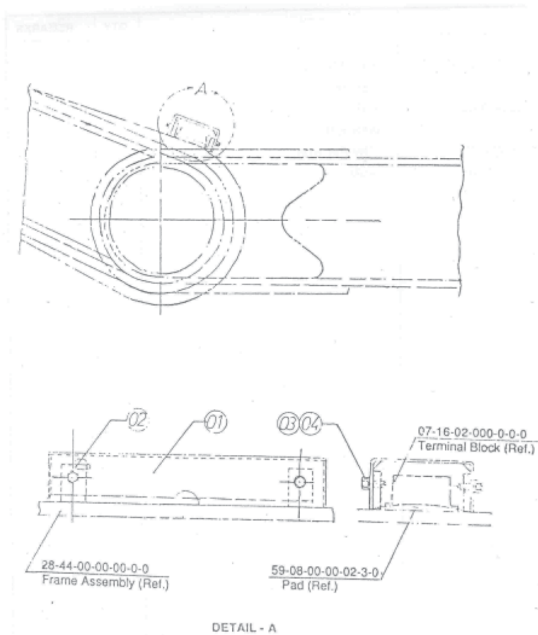
FIG NO. 150 COVER INSTALLATION (OPTIONAL)
