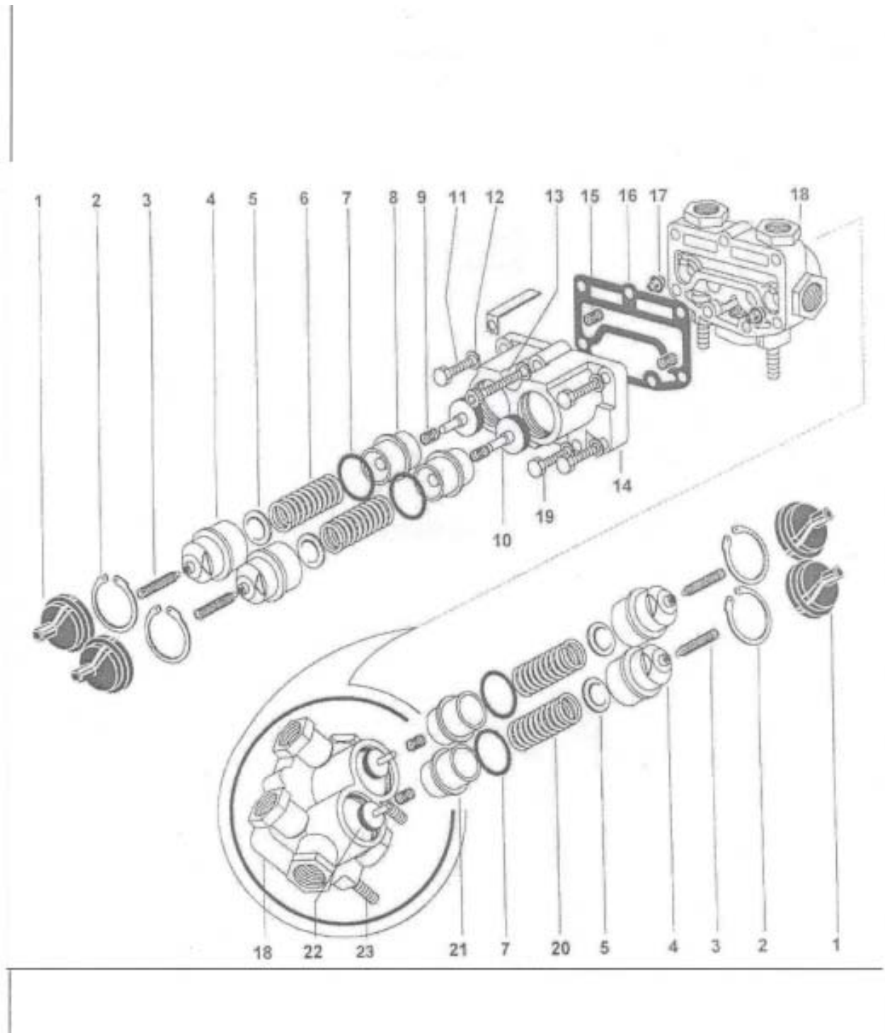
FIG NO. 60C SYSTEM PROTECTION VALVE
