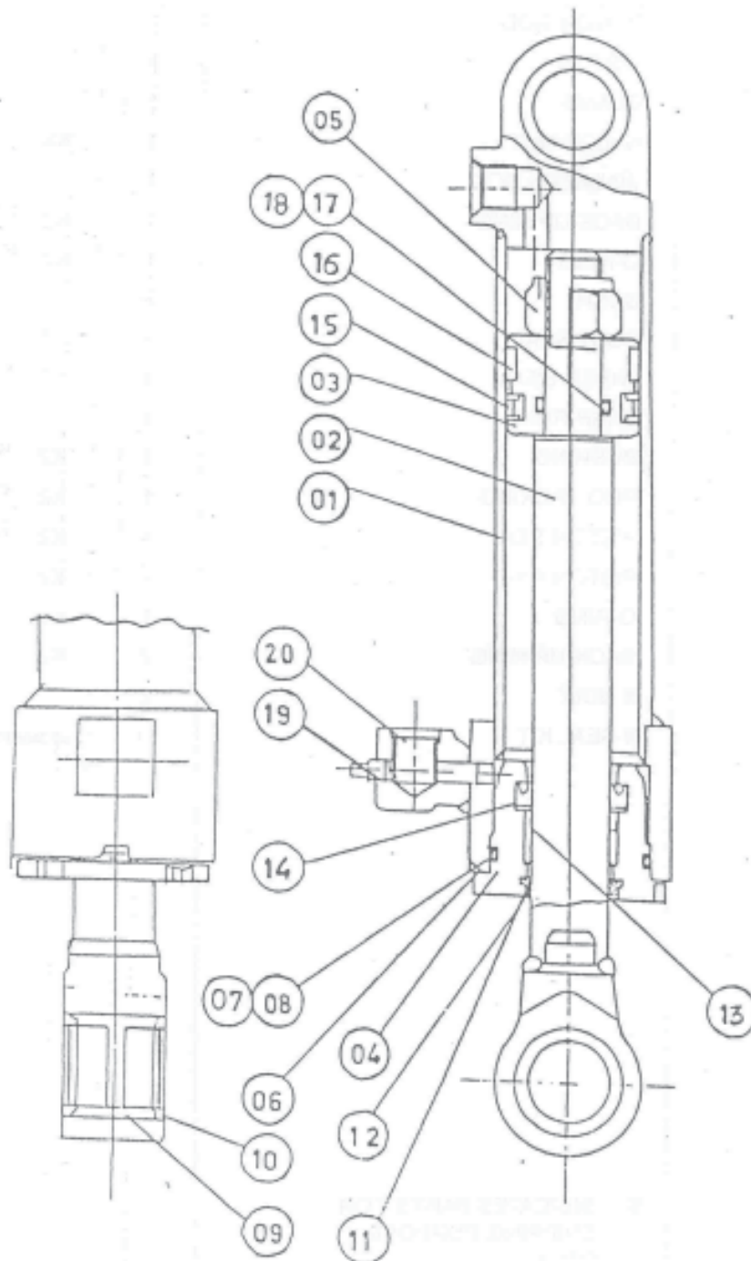
FIG NO. 89 STEERING CYLINDER
