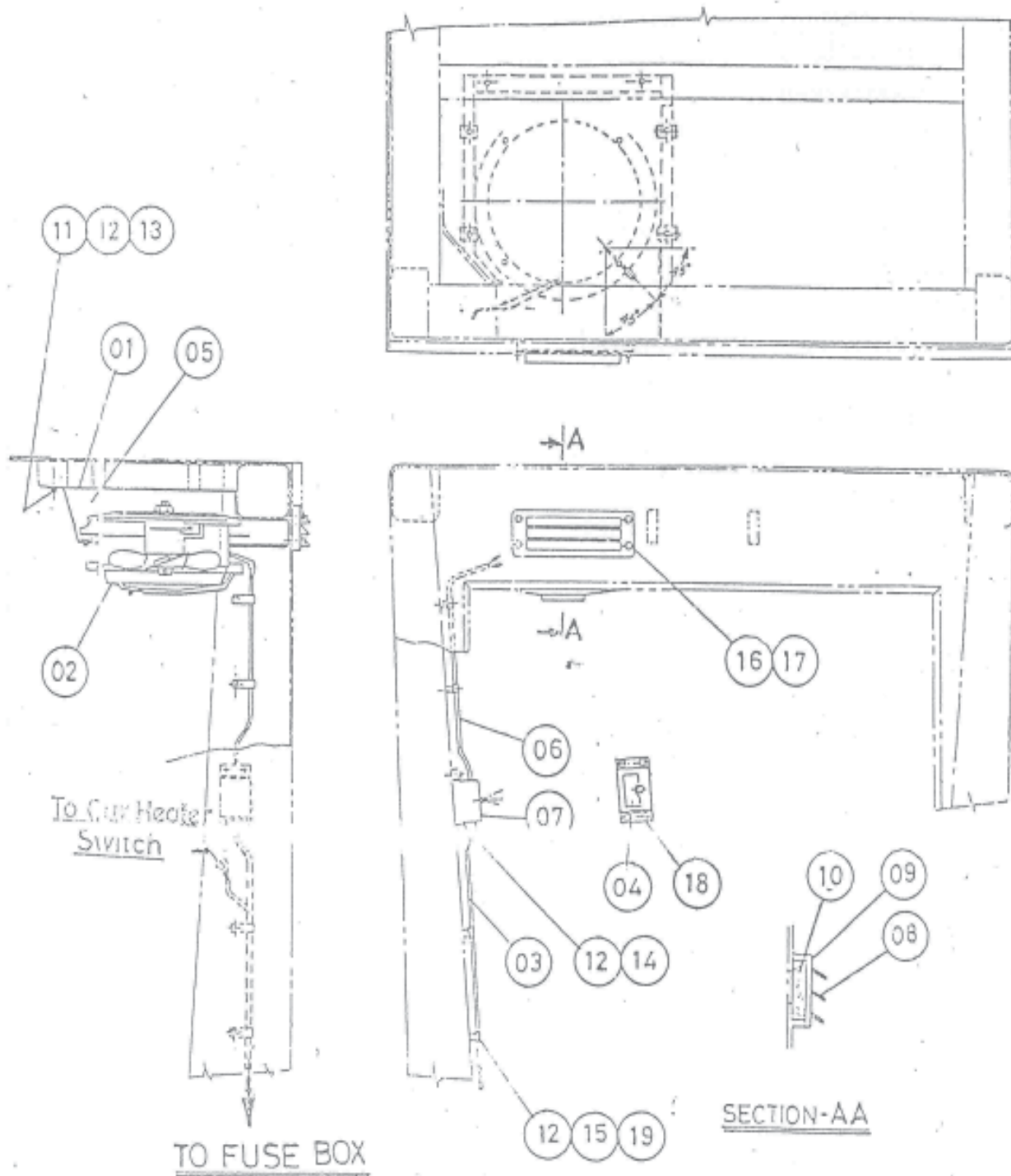
FIG NO.139 VENTILATORASSEMBLY (OPTIONAL)
