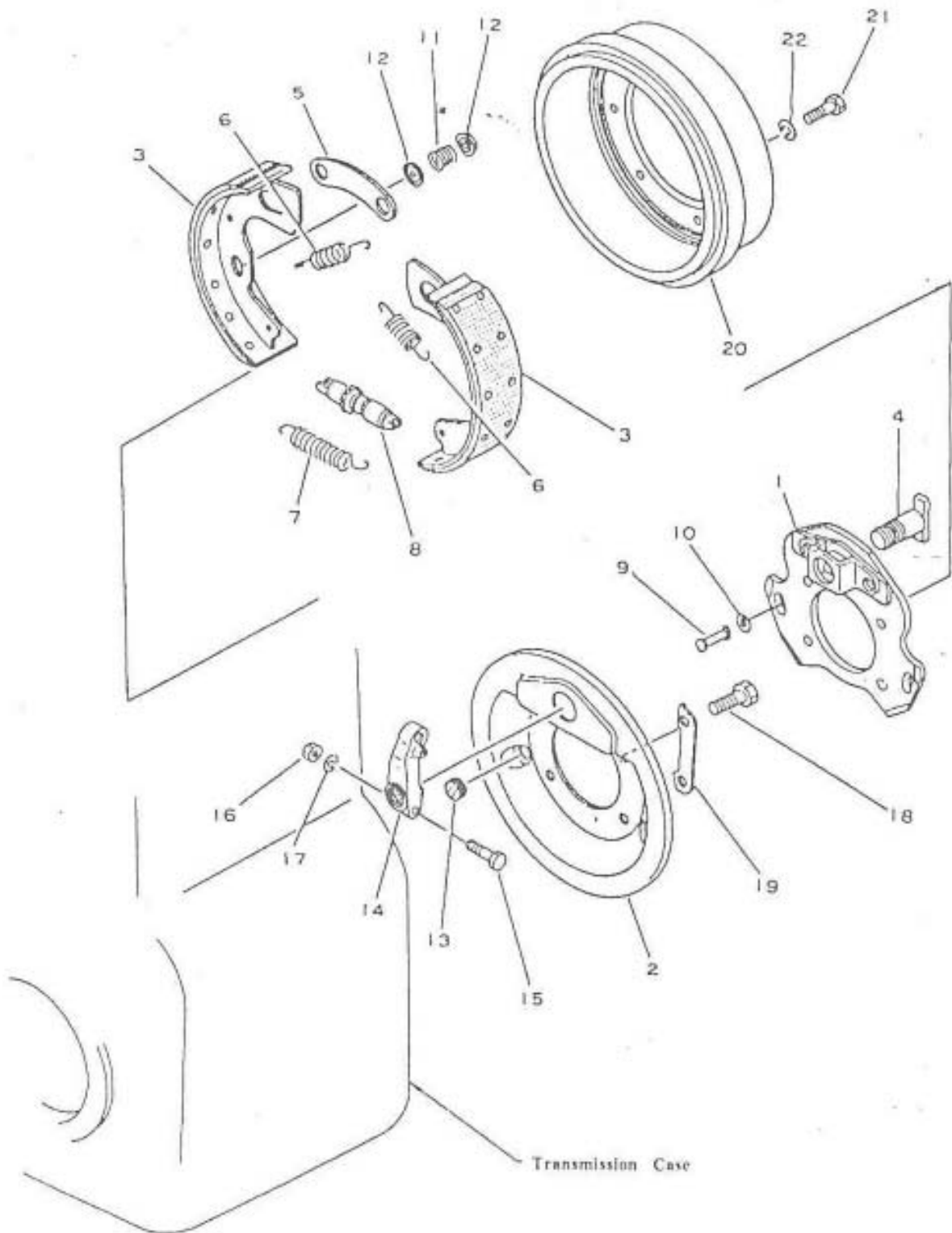
FIG NO. 60 PARKING BRAKE
