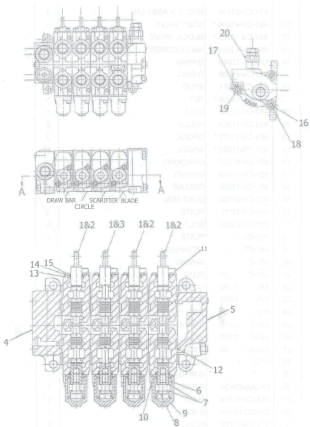
SECTIONAL VIEW
